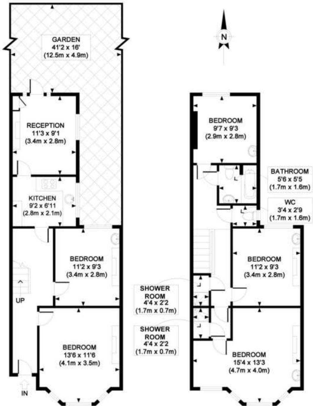
GROUND FLOOR GROSS INTERNAL FLOOR AREA 529 SQ FT
